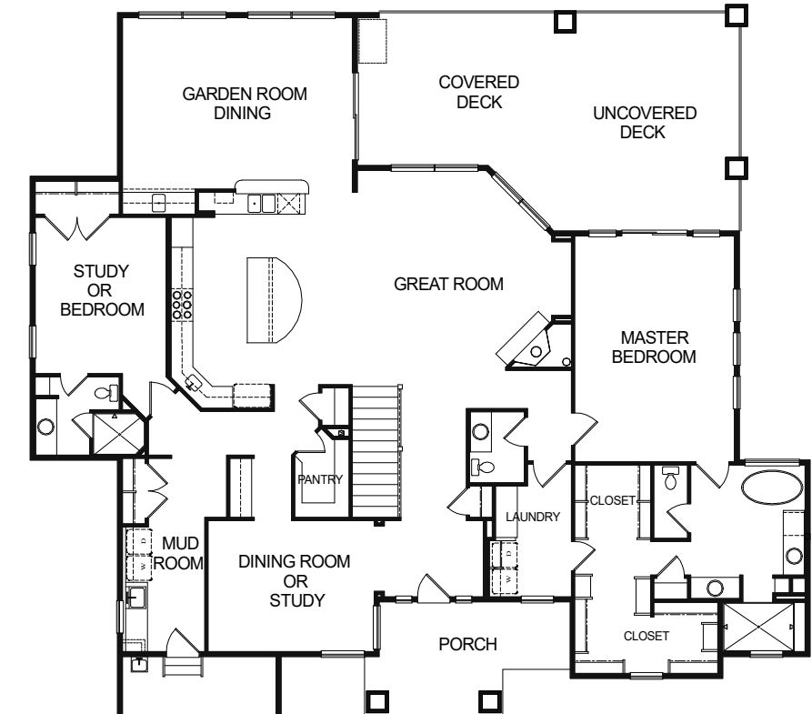
MAIN LEVEL
